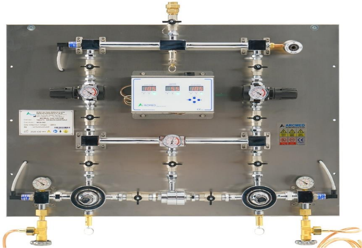
OXYGEN AUTOMATIC MANIFOLD
