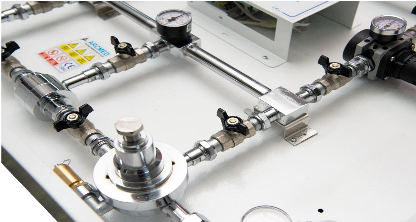
NITROUX OXIDE STANDBY MANIFOLD
